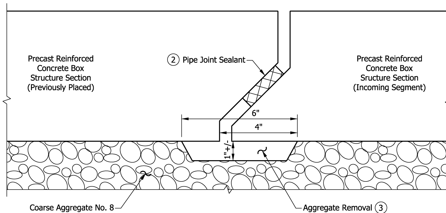
SECTION THROUGH BOTTOM OF BOX STRUCTURE
