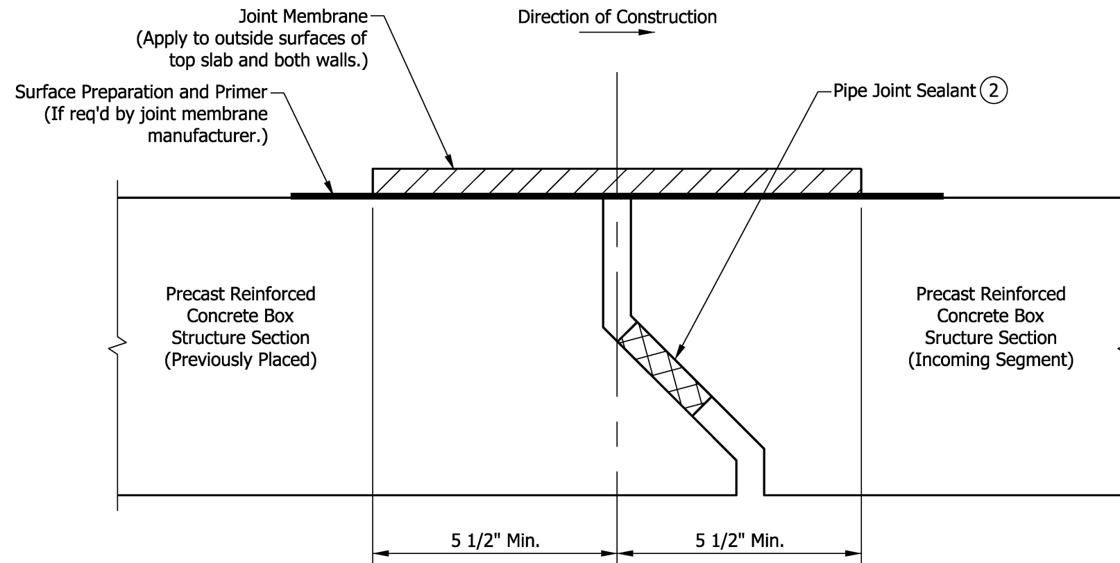
SECTION THROUGH TOP OF BOX STRUCTURE
